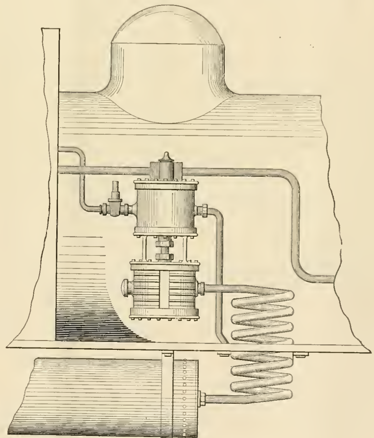
PROPOSED COOLING PIPE FOR AIR PUMPS.
